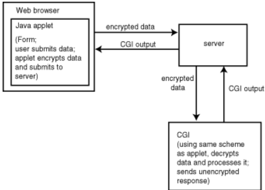
Figure 9.4 : An applet sends the form data instead of the browser.
