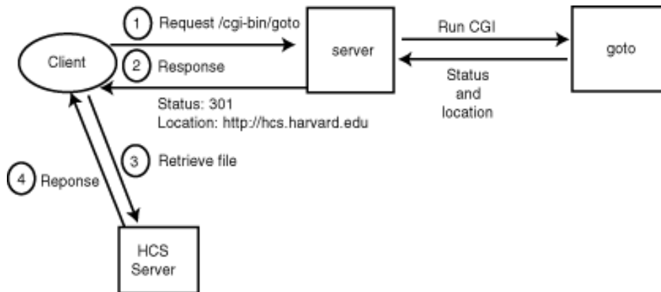
Figure 8.8 : Redirection request for a file that has temporarily moved.
