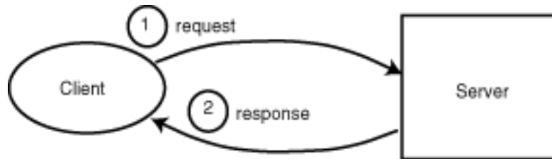
Figure 8.2 : The HTTP request/response paradigm.
