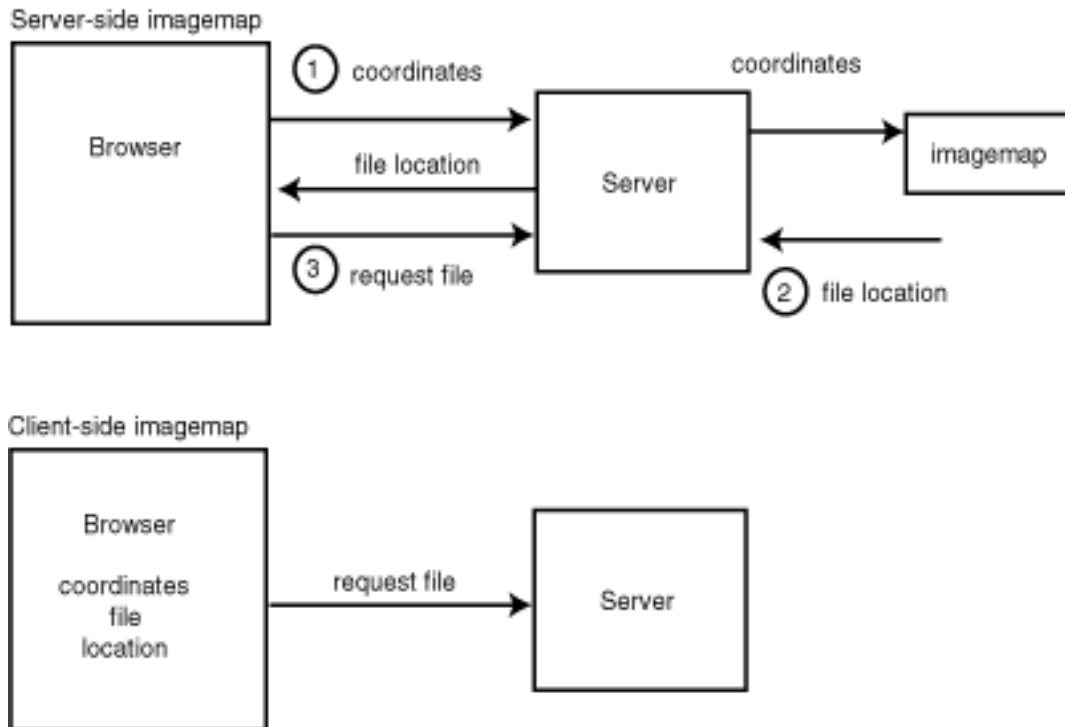
Figure 14.1 : Using an imagemap CGI application requires the browsers to make two connections to the server. A client-side imagemap requires only one connection.
