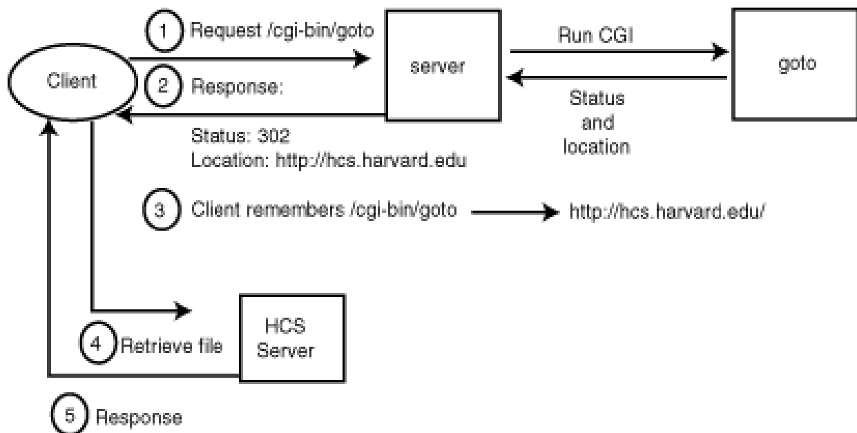
Figure 8.9 : Redirection request for a file that has permanently moved.
