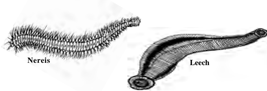
Fig. 1.2.11 Annelids
