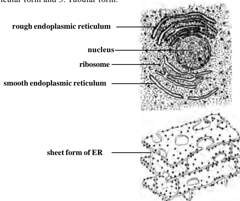
Fig.2.2.6. Endoplasmic reticulum
