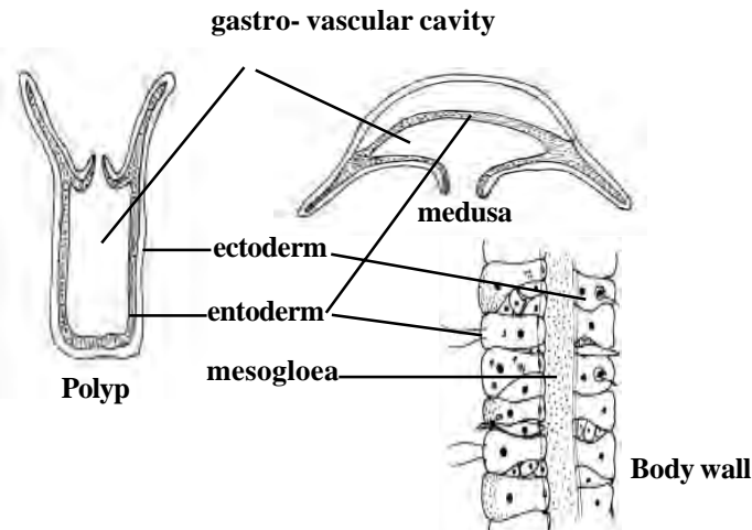
Fig. 1.2.4 Coelenterate-body wall
