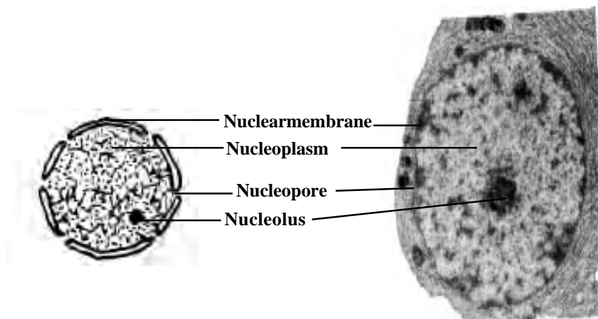
Fig.2.2.9. Nucleus
