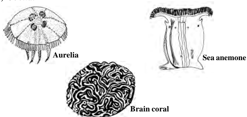
Fig. 1.2.6 Coelenterates
